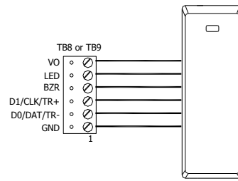
Typical 2-Wire RS-485 Device
